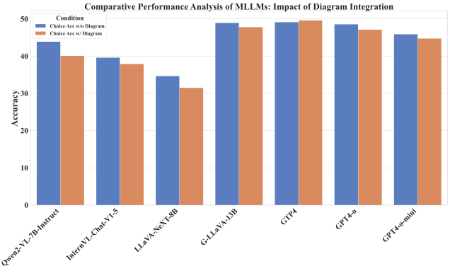
Fig. 1. Comparative performance analysis of MLLMs: Impact of diagram integration
